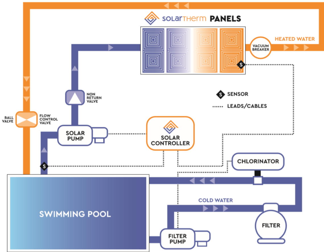
Diagram 1: Pool plumbed for solar heating.
