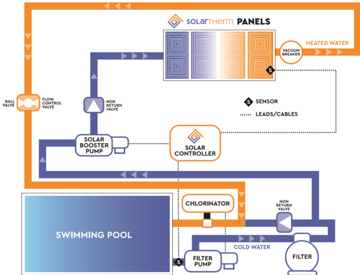
Diagram 2: Pool not plumbed for solar heating.
